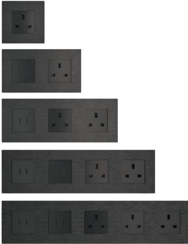
SQUARE 6mm 45x45 insert Legrand Arteor/Mosaic/Valena Next , Peha Concept 45 , Simon K45 , Hager Gallery, Efapel MEC Q45, Sinoamigo type 45, TEM teknik, Niko (RJ45 only) All metals
